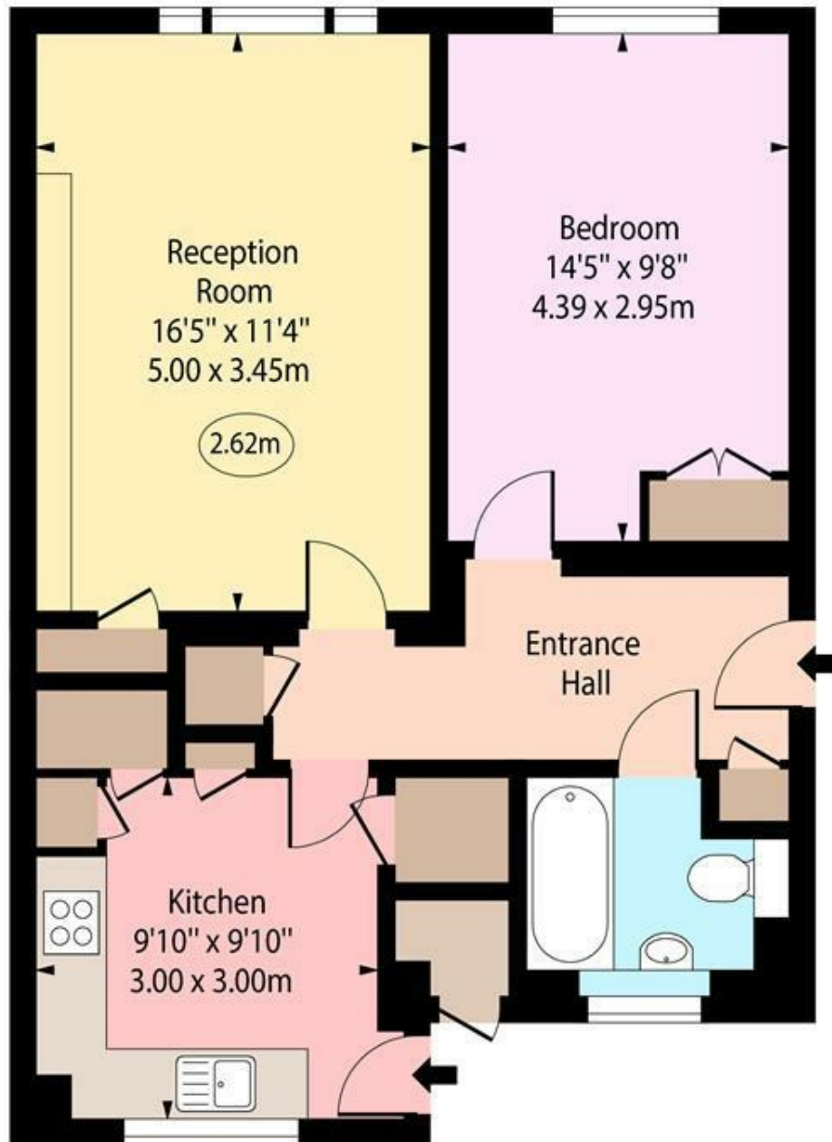
Ground Floor
